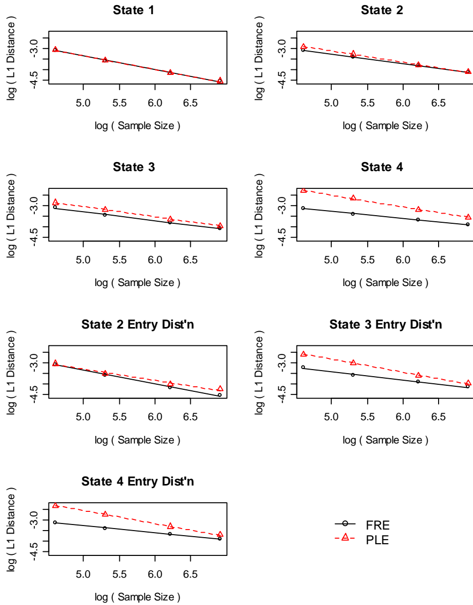
Figure for Table 8: The log mean L1 distances of state occupation probabilities and state entry/exit time distributions in a four-state Markov tracking simulation model with Lognormal state waiting times and Weibull censoring times.
