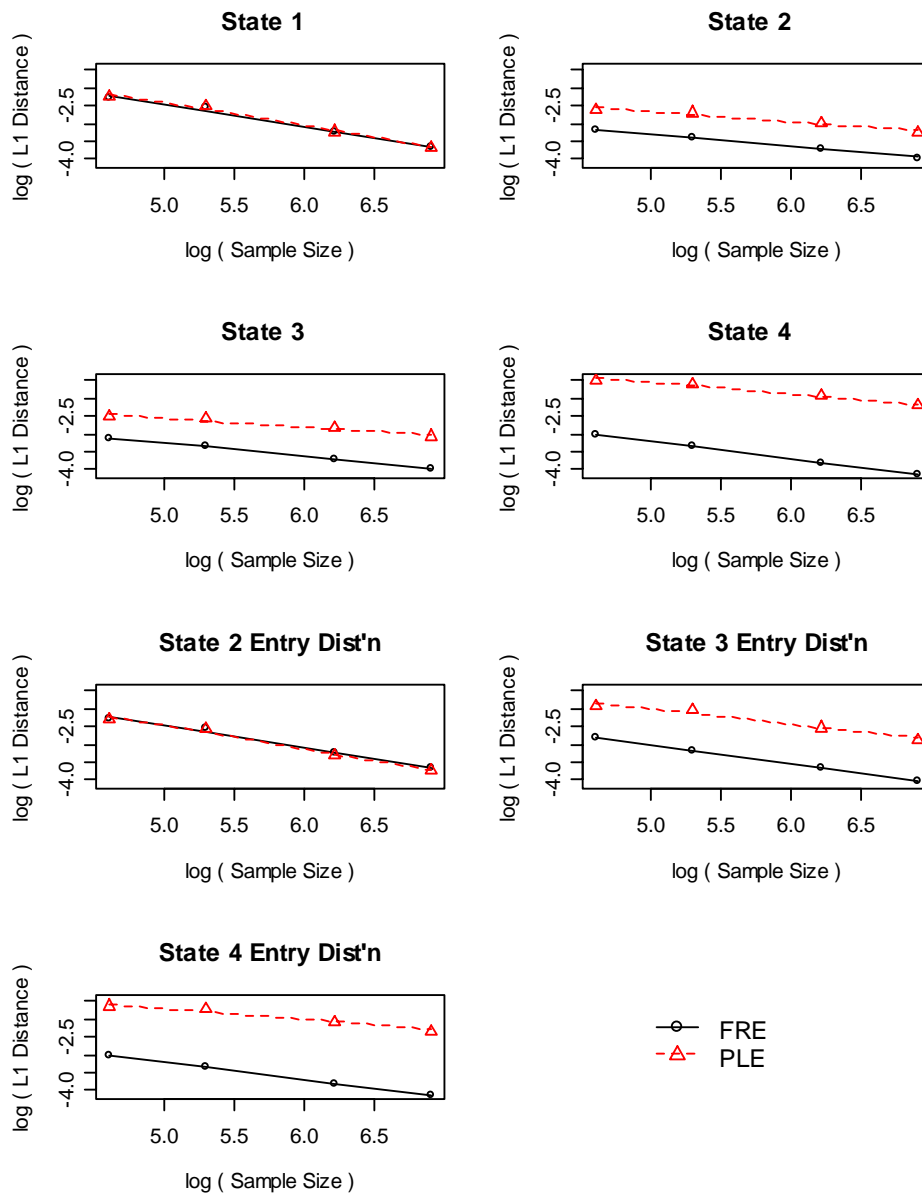
Figure for Table 4: The log mean L1 distances of state occupation probabilities and state entry/exit time distributions in a four-state Markov tracking simulation model with Weibull state waiting times and Weibull censoring times
